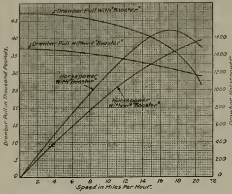
FIG. 1. DRAWBAR PULL VS. SPEED CURVE NEW YORK CENTRAL CLASS K. L. E. LOCOMOTIVE
